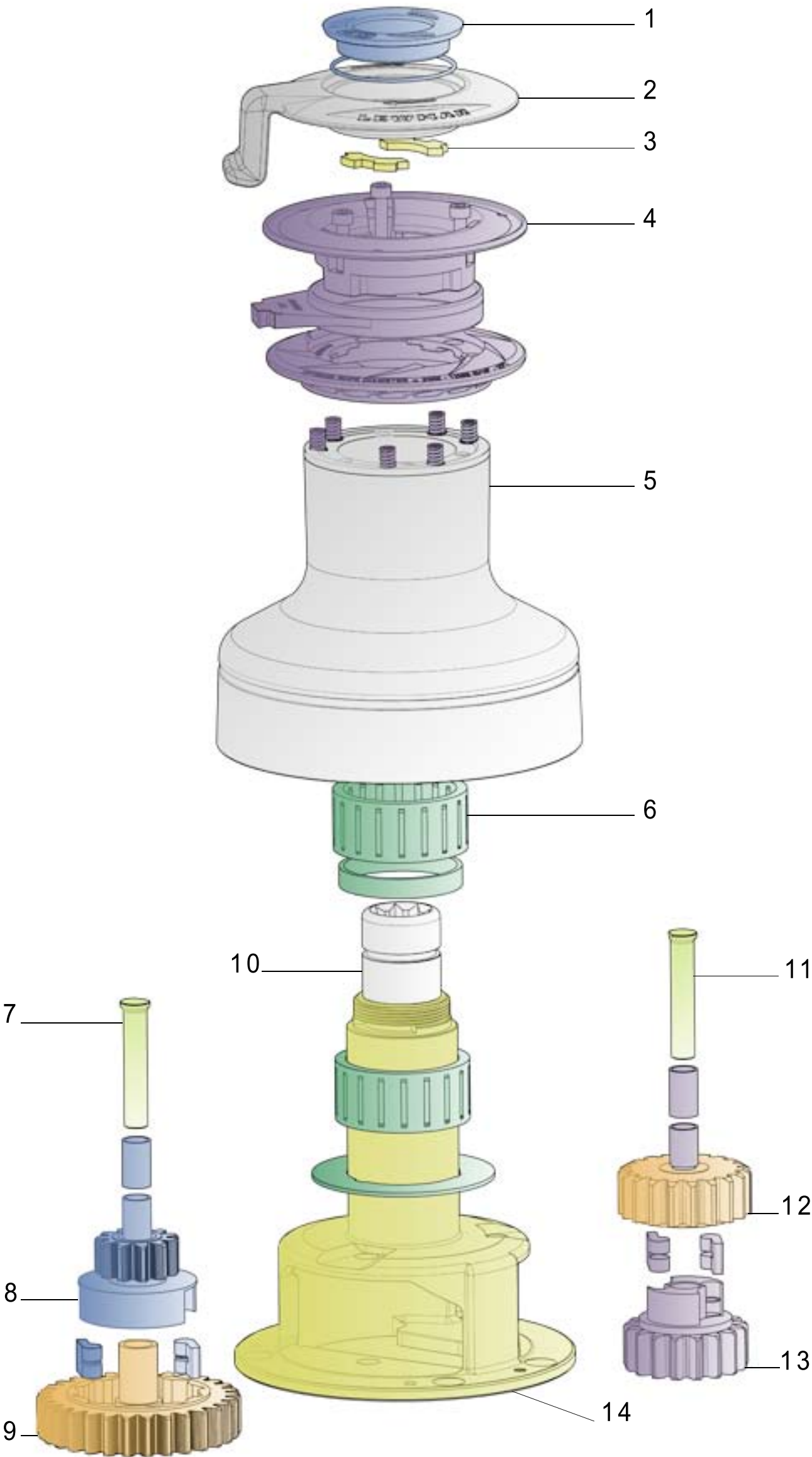
Evo Size 30/40/45/50 exploded view
