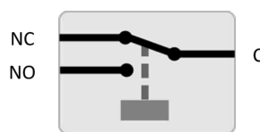
Relay configuration (not energised).
